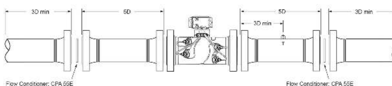
Figure 15: Piping Recommendation for Bi-directional Gas Ultrasonic Meter with Flow Conditioners (Compact Installation) (10)
