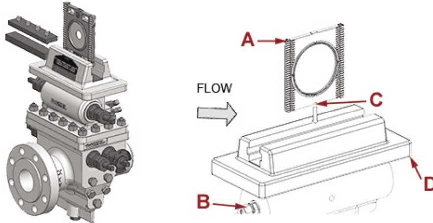
Figure 3: Orientation of plate carrier prior to installation
